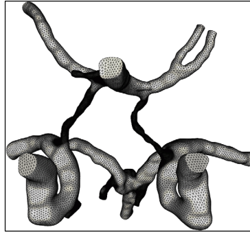
Figure 2b Circle of Willis: Surface Mesh
