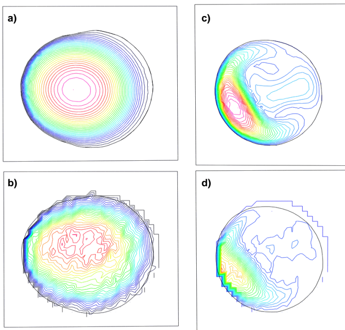
Figure 1b Phantom: Comparison of Velocities (CFD-MRA)
