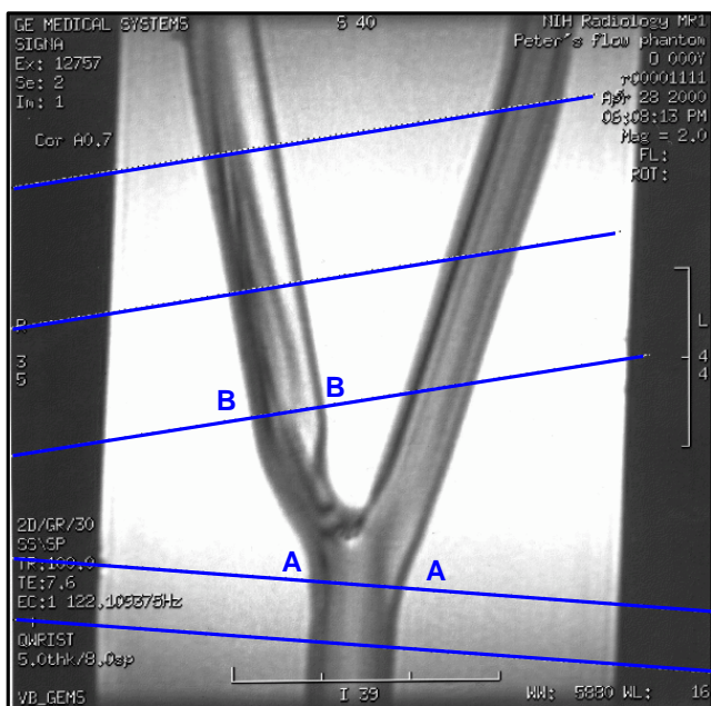
Figure 1a Phantom: MIP Geometry Definition and MRA Cuts
