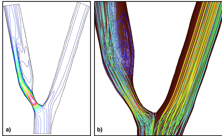
Figure 1c Phantom: Abs(Vel) in Plane and Streamlines
