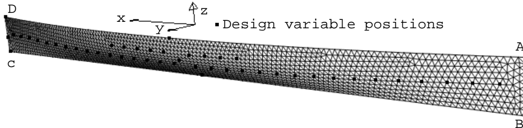
Figure 1. Surface mesh of the Wigley hull
