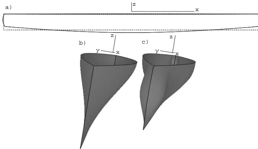
Figure 3. a) Initial hull (dashed line) and final hull (continuous line) b) Initial hull c) Final hull
